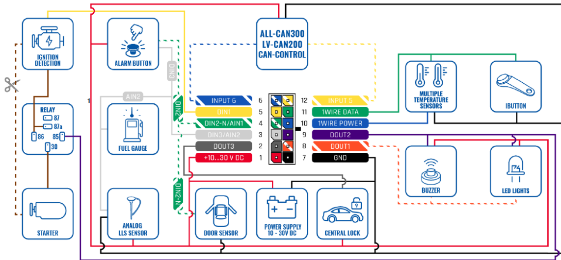
Figure 3 FMC130 Wiring scheme
